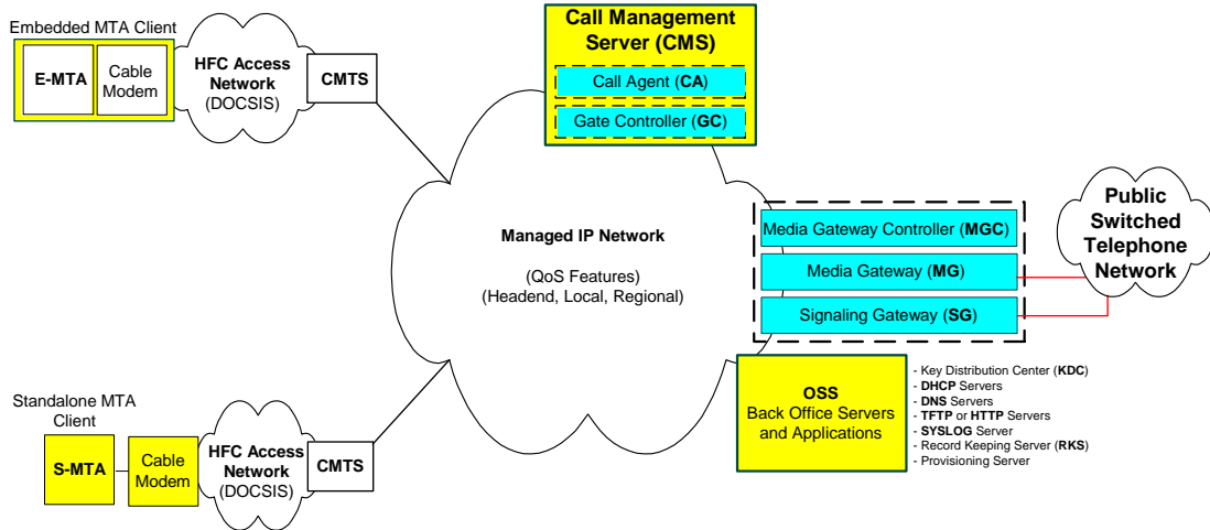
Figure 2. PacketCable 1.0 Network Component Reference Model (partial)
