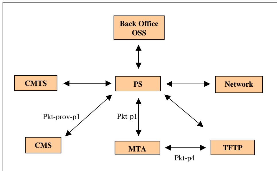
Figure 3. Provisioning Component Interfaces
