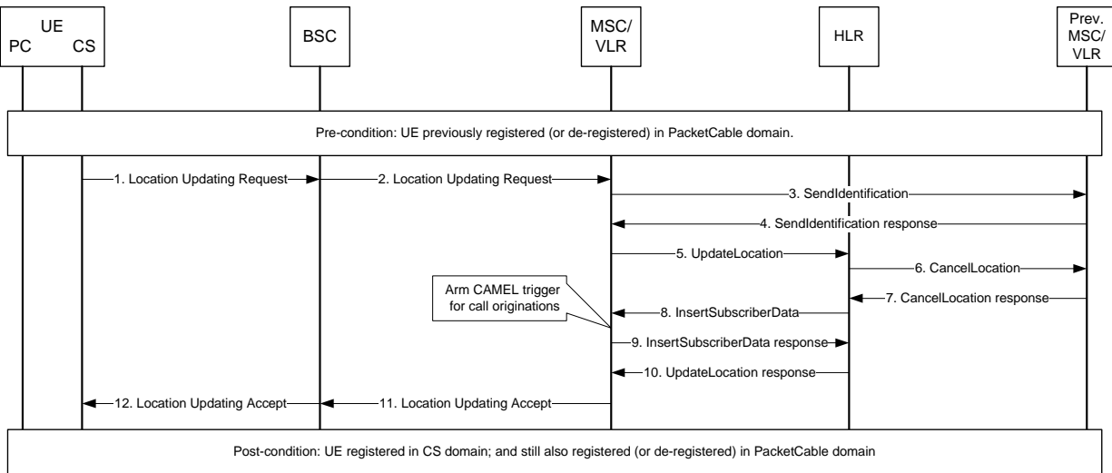
Figure 14 - UE Registration in CS Domain (3GPP)
