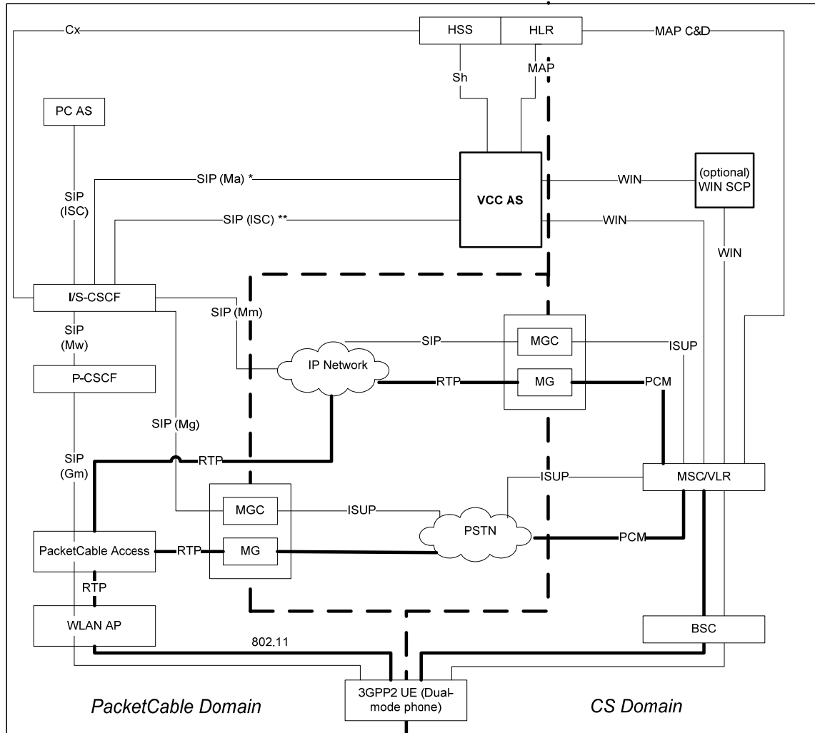
Figure 2 - PacketCable Interfaces to 3GPP2 Circuit Cellular Networks
