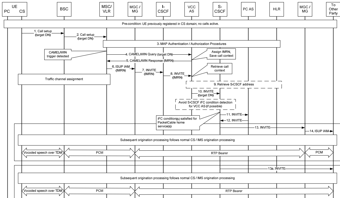
Figure 16 - UE Origination Call Setup in CS Domain
