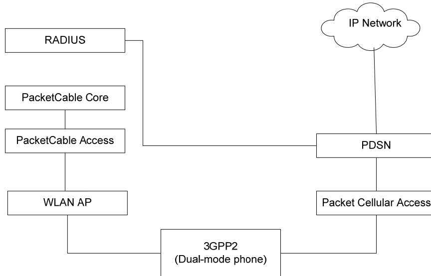
Figure 4 - PacketCable Interfaces to 3GPP2 Packet Cellular Networks
