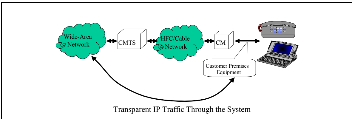
Figure 1. Transparent IP Traffic Through the Data-Over-Cable System
