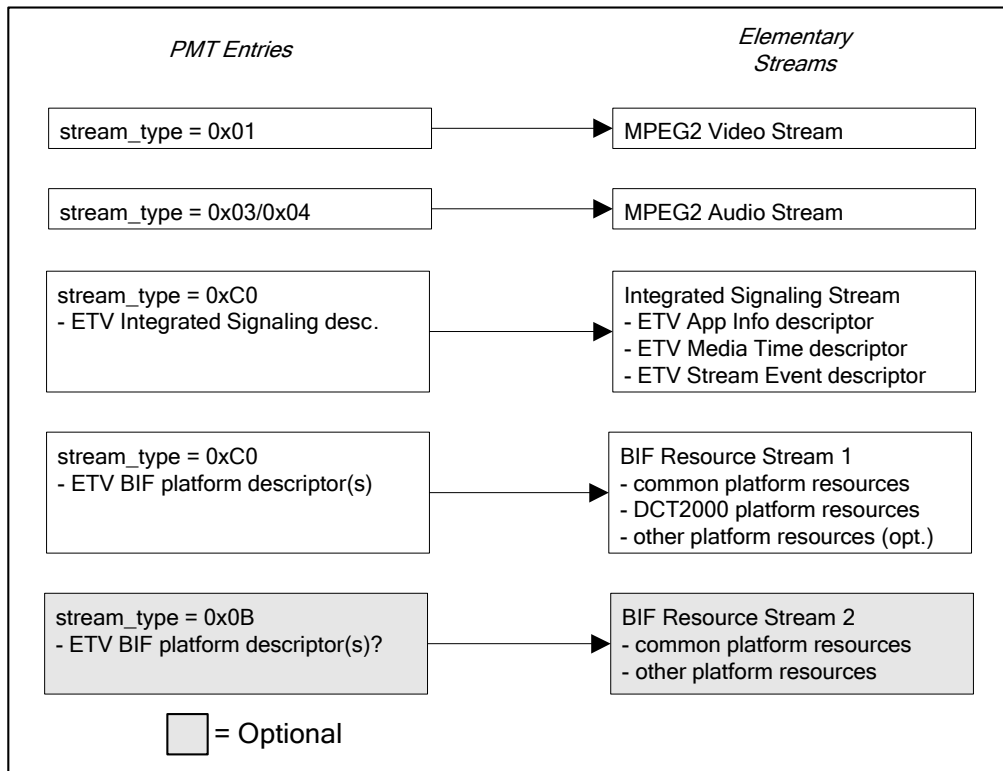
Figure 9-1 - PMT Signaling Motorola DCT-2000 Specific Behaviors
