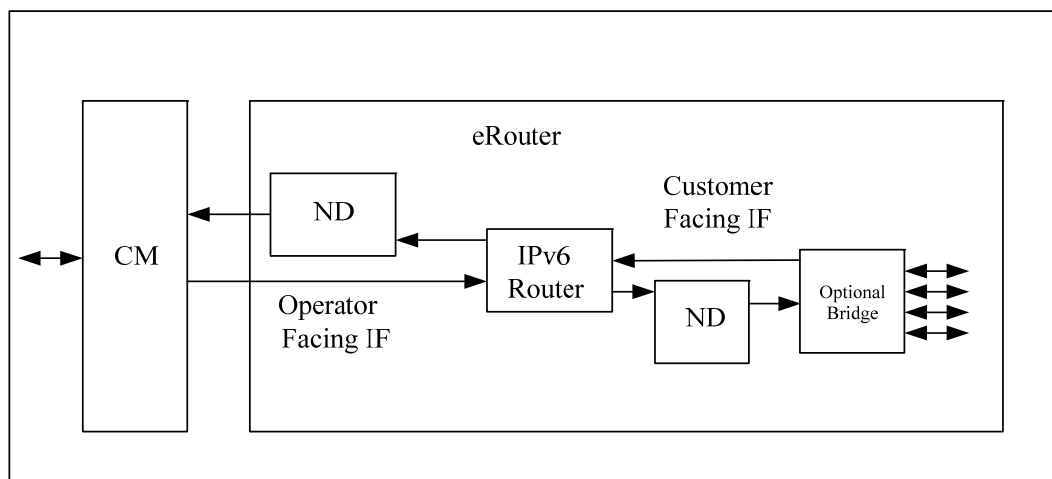
Figure 10-1 - eRouter IPv6 Forwarding Block Diagram
