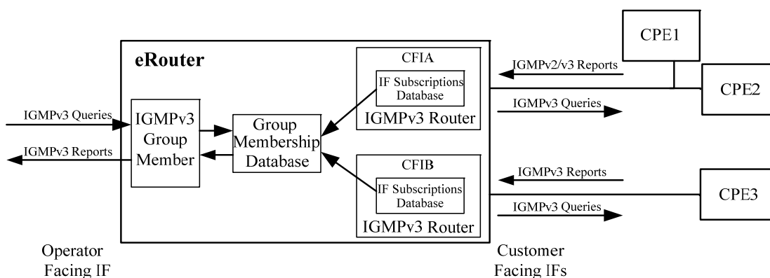
Figure 9-3 - IPv4 Multicast Forwarding Example 16
