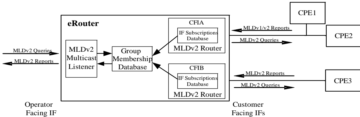
Figure 10-3 - IPv6 Multicast Forwarding Example 24
