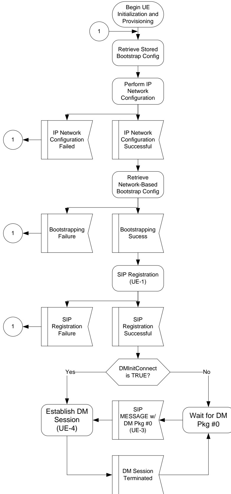
Figure 8 - UE Provisioning Flow
