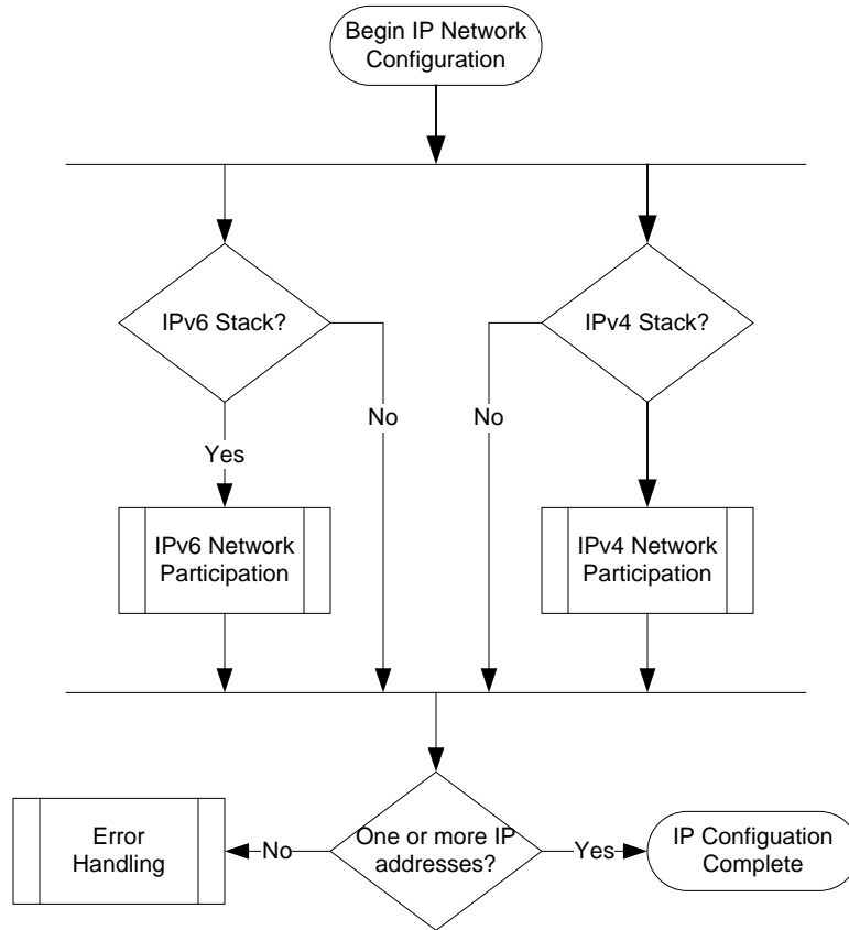
Figure 6 - IP Network Configuration (UE)
