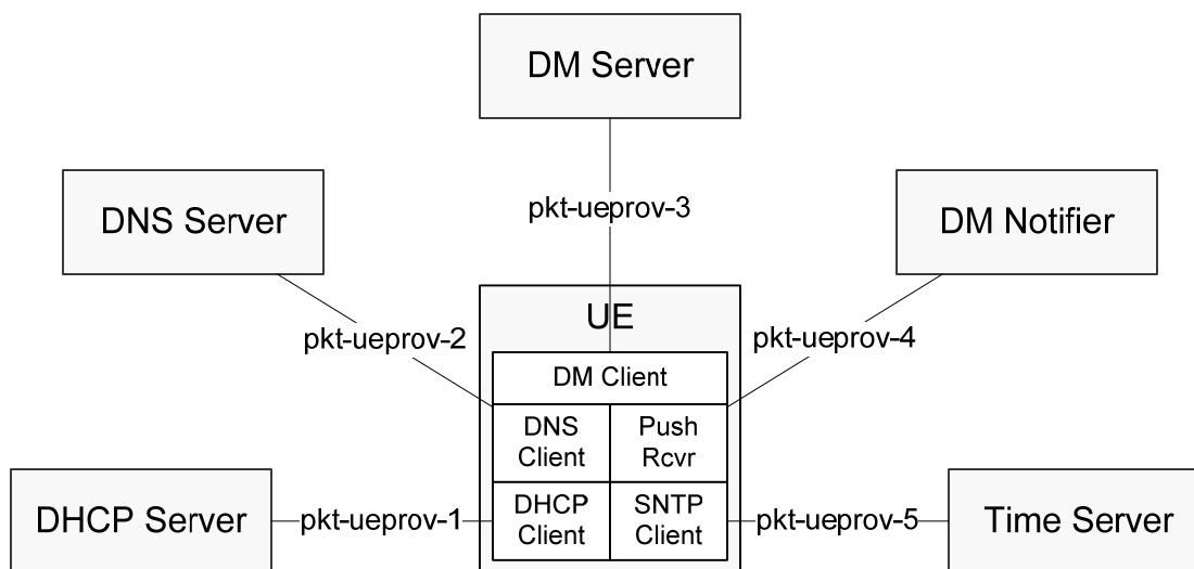
Figure 4 - UE Provisioning Interfaces (logical view)
