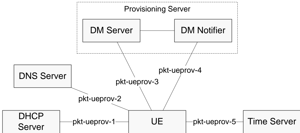
Figure 5 - UE Provisioning Components and Interfaces
