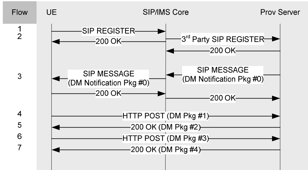
Figure 10 - Example Provisioning Flow
