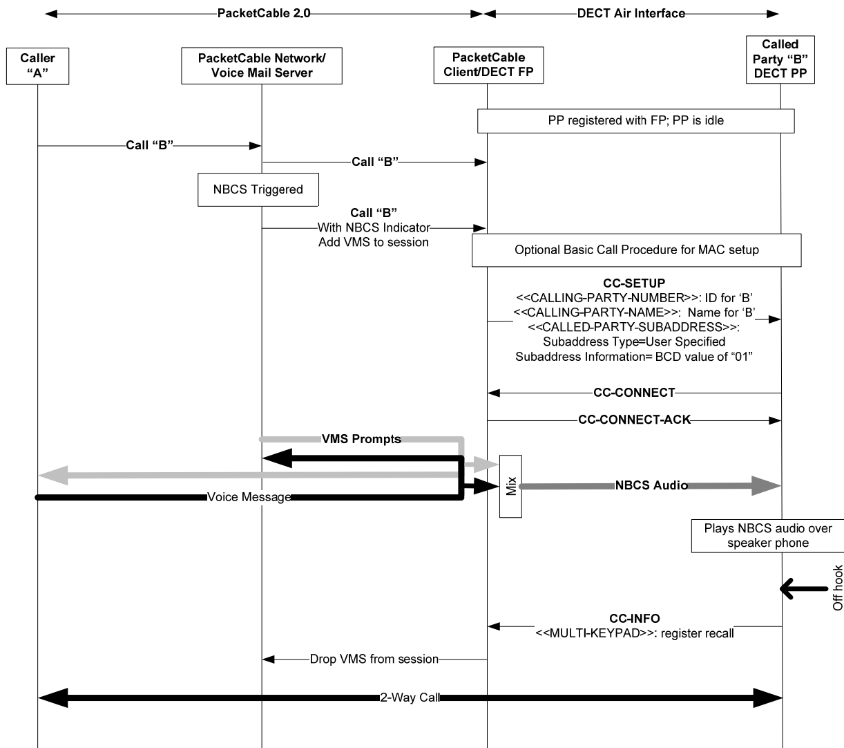
Figure 5 - Network Based Call Screening Call Flow Example
