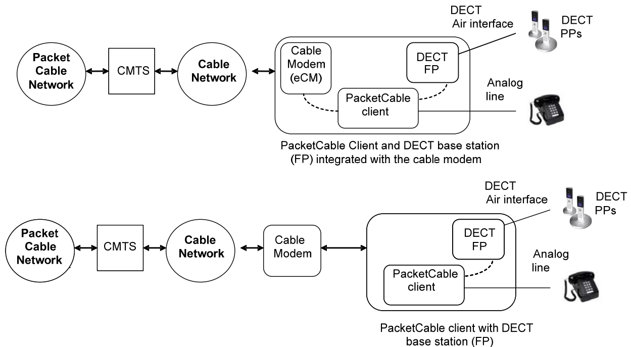
Figure 1 - PacketCable Clients with HD Voice via DECT
