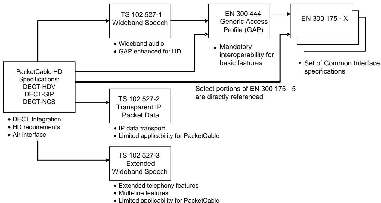
Figure 4 - Leveraging DECT for HD Voice
