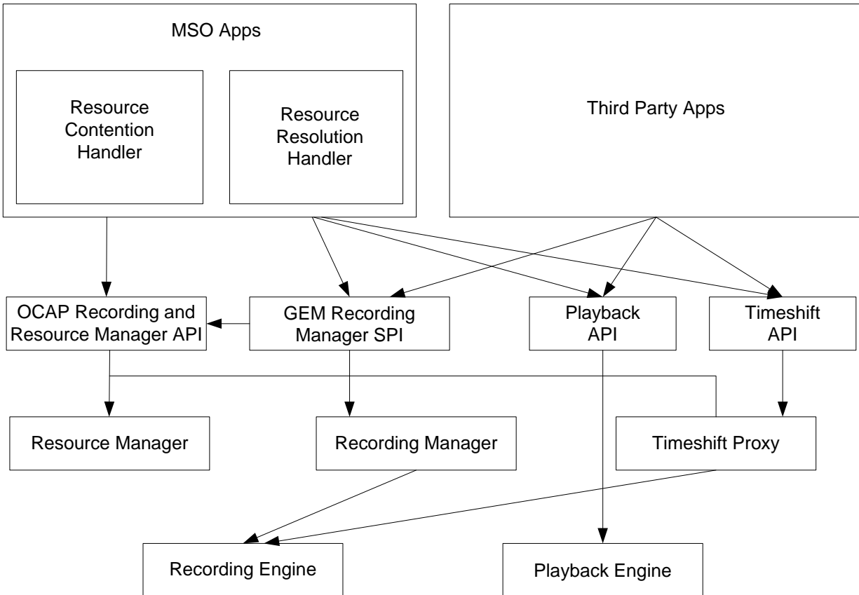
Figure 5-1 - DVR Architecture
